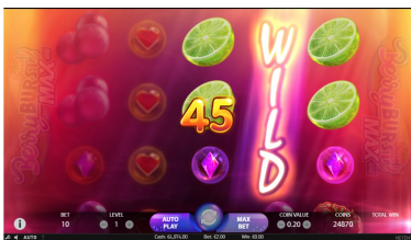
Expanding-Wild-Symbole
