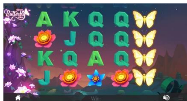
Re-Spins activation
